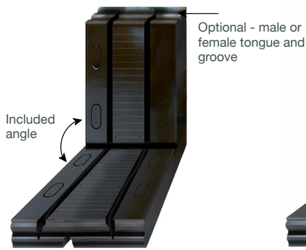
Examples of a factory vulcanised kerb unit for models 150, 200, 250 & 300
