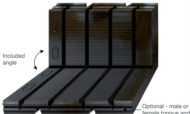
Examples of a factory vulcanised kerb unit for models 400, 650, 900 & 1300
